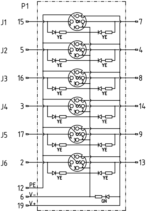
WIRING DIAGRAM
